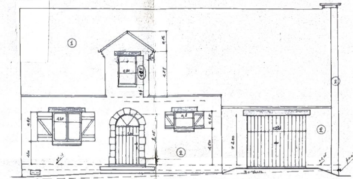
FAÇADE PRINCIPALE
