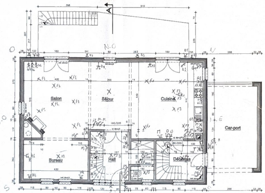
PLAN REZ
